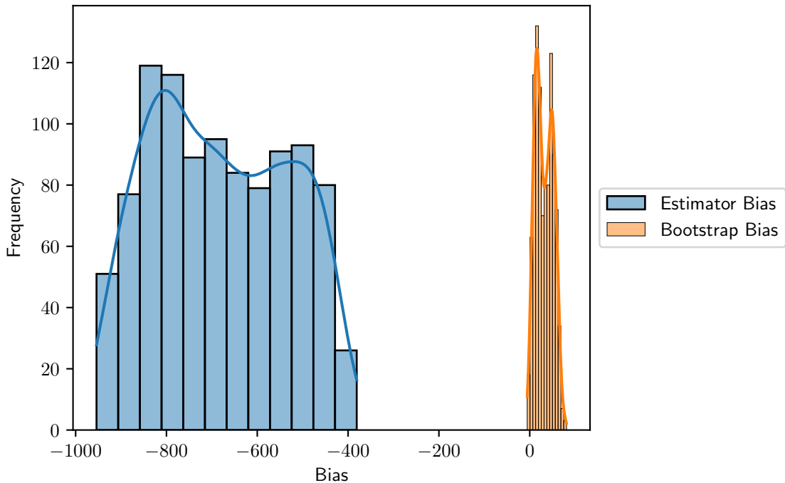
Distribution of Bias_Uterus
